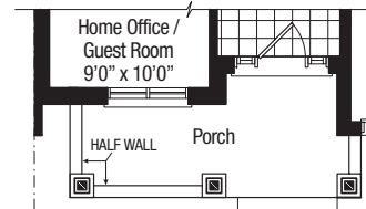
First Floor Plan Part Elevation B
