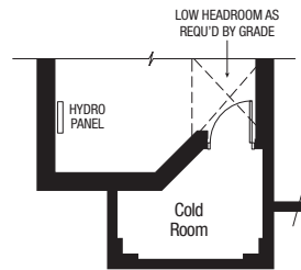
Part Basement Floor Plan Elevation B
