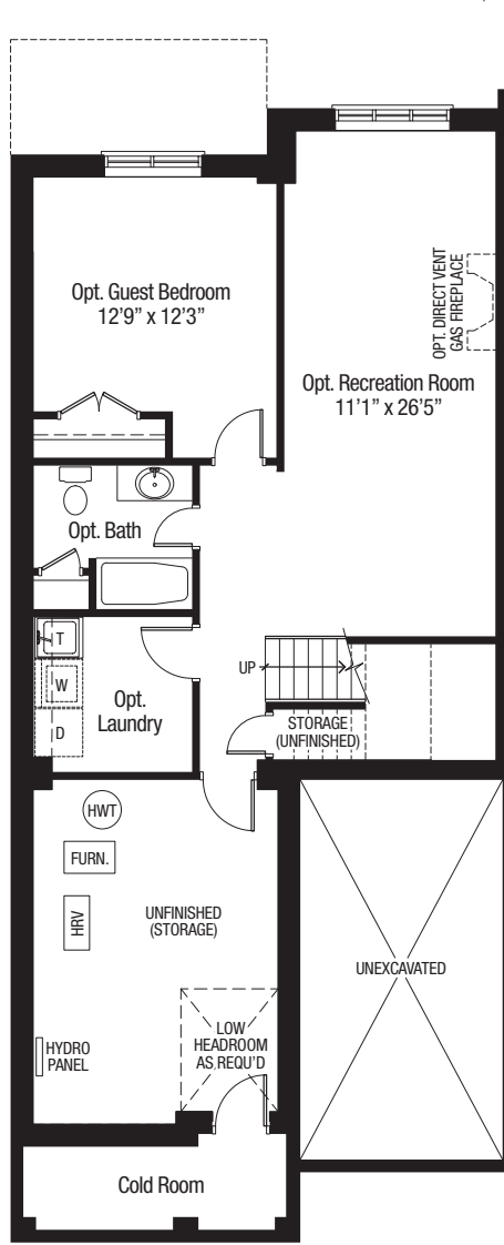
Part Basement Floor Plan Elevation B
