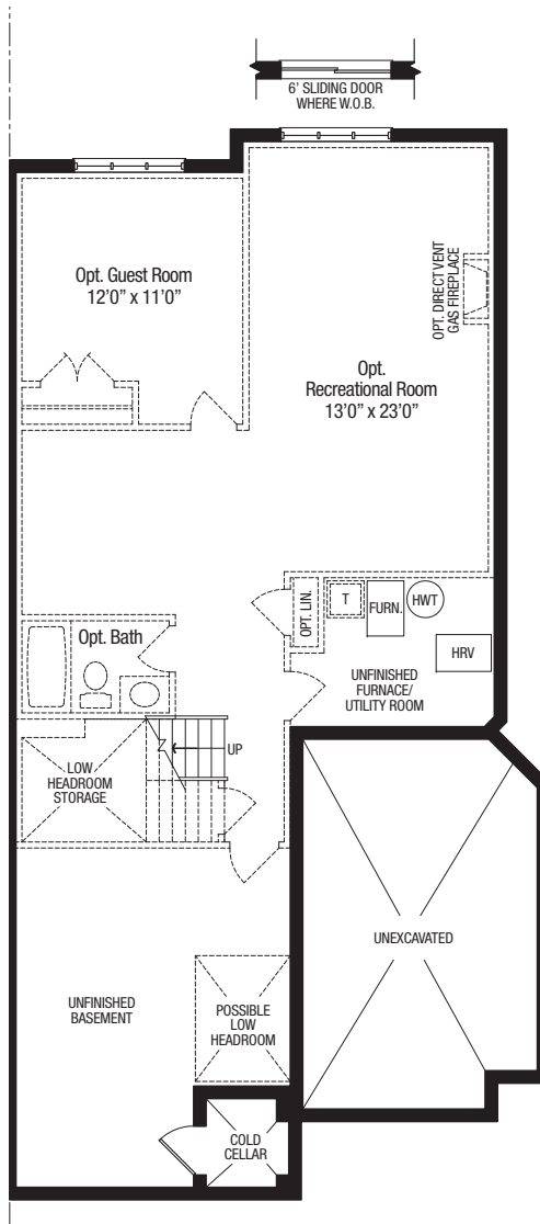
Basement Floor Plan Elevation A & B
