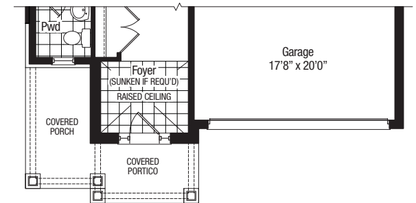
First Floor Plan Elevation B
