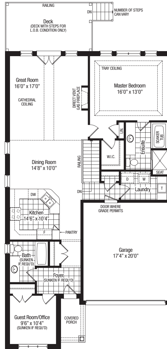
First Floor Plan Elevation A & B
