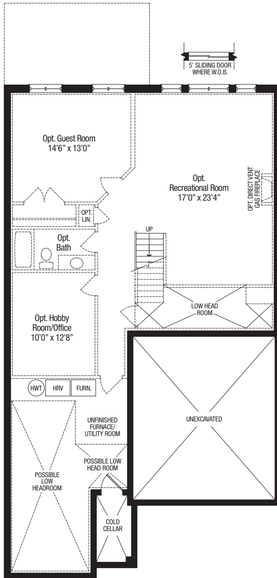
Basement Floor Plan Elevation A & B
