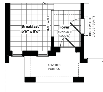
FIRST FLOOR Plan Elevation B
