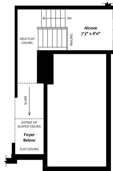
ALCOVE FLOOR Plan Elevation A & B
