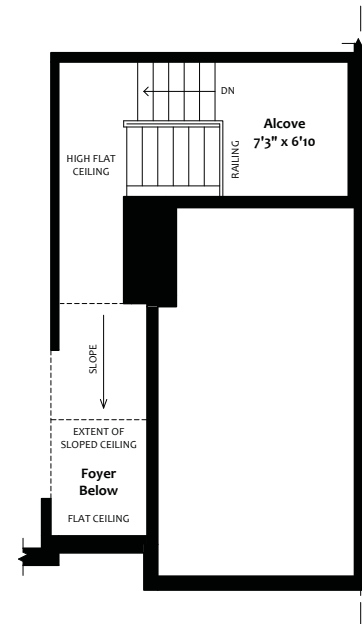
ALCOVE FLOOR Plan Elevation A & B
