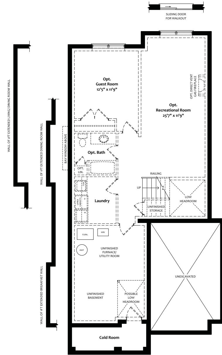
LOWER LEVEL Plan Elevation A
