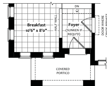
FIRST FLOOR Plan Elevation B
