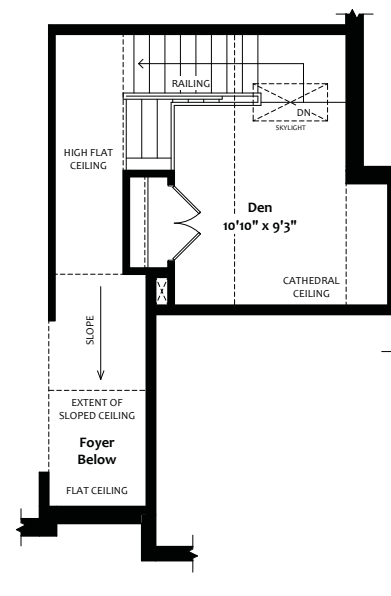
LOFT FLOOR Plan Elevation A & B
