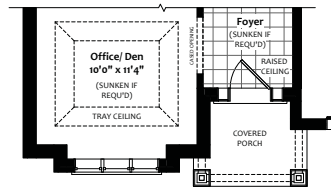
FIRST FLOOR Plan Elevation B
