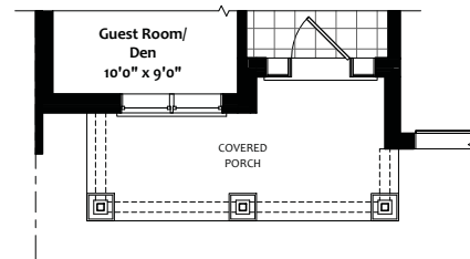
FIRST FLOOR Plan Elevation B
