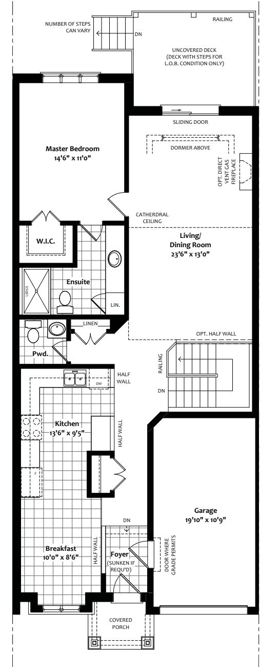
FIRST FLOOR Plan Elevation A
