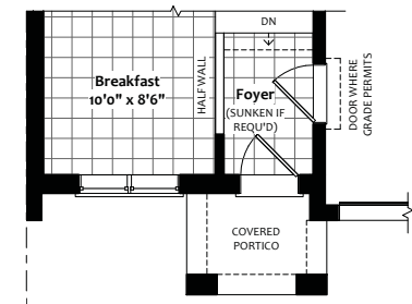
FIRST FLOOR Plan Elevation B
