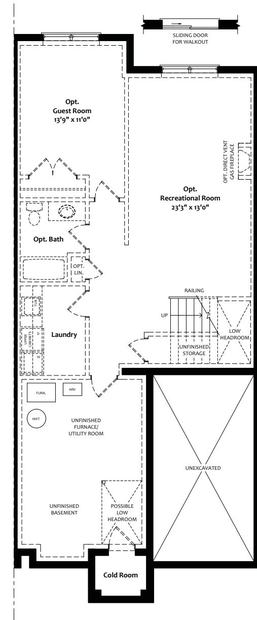
LOWER LEVEL Plan Elevation A
