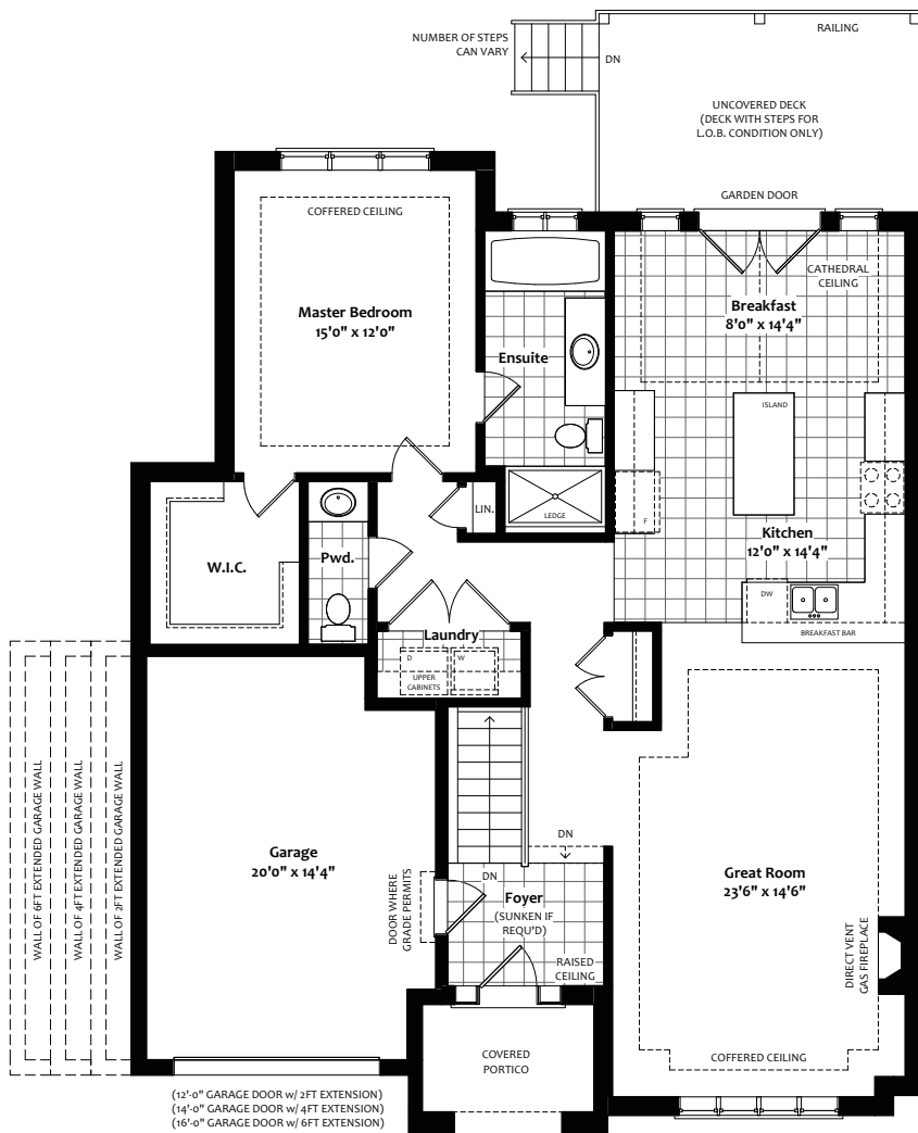
FIRST FLOOR Plan Elevation A
