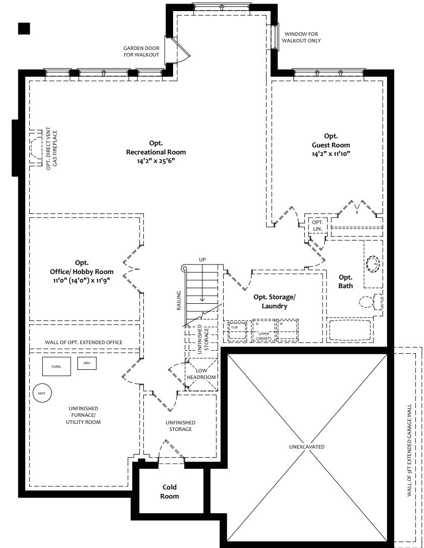
LOWER LEVEL Plan Elevation A & B
