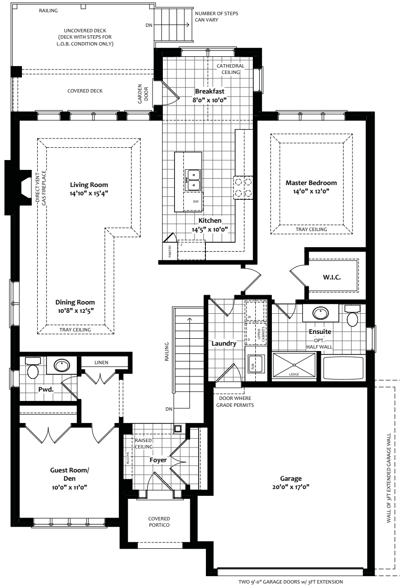
FIRST FLOOR Plan Elevation A
