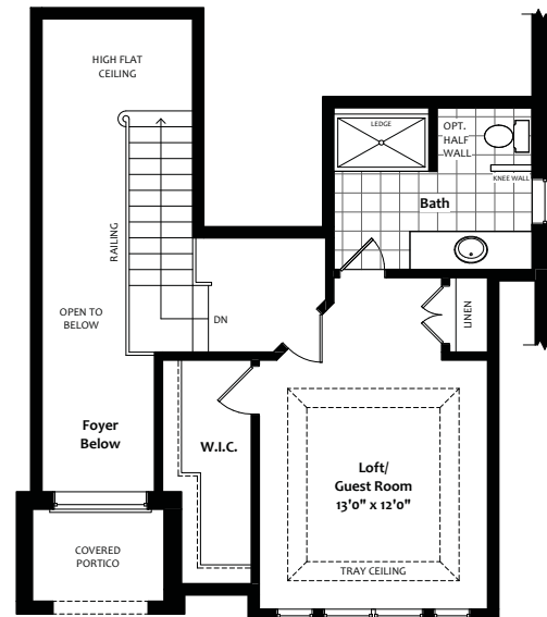
LOFT FLOOR Plan Elevation A
