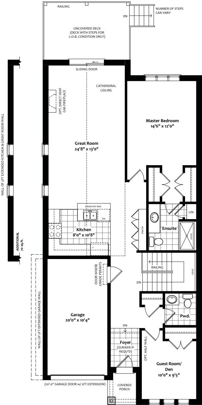
FIRST FLOOR Plan Elevation A
