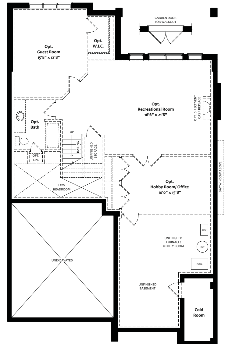
LOWER LEVEL Plan Elevation A
