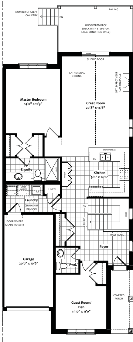
FIRST FLOOR Plan Elevation A
