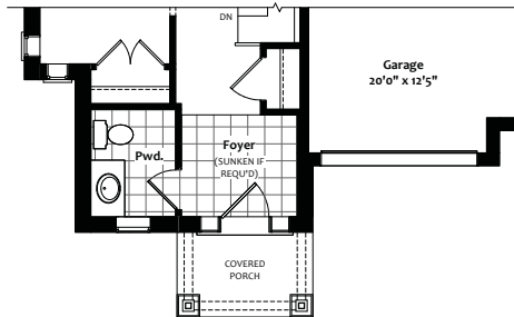
FIRST FLOOR Plan Elevation B
