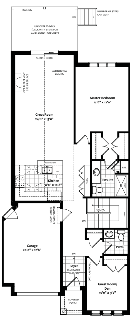
FIRST FLOOR Plan Elevation A
