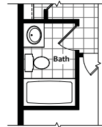
FIRST FLOOR Opt. Bath Plan Elevation A & B
